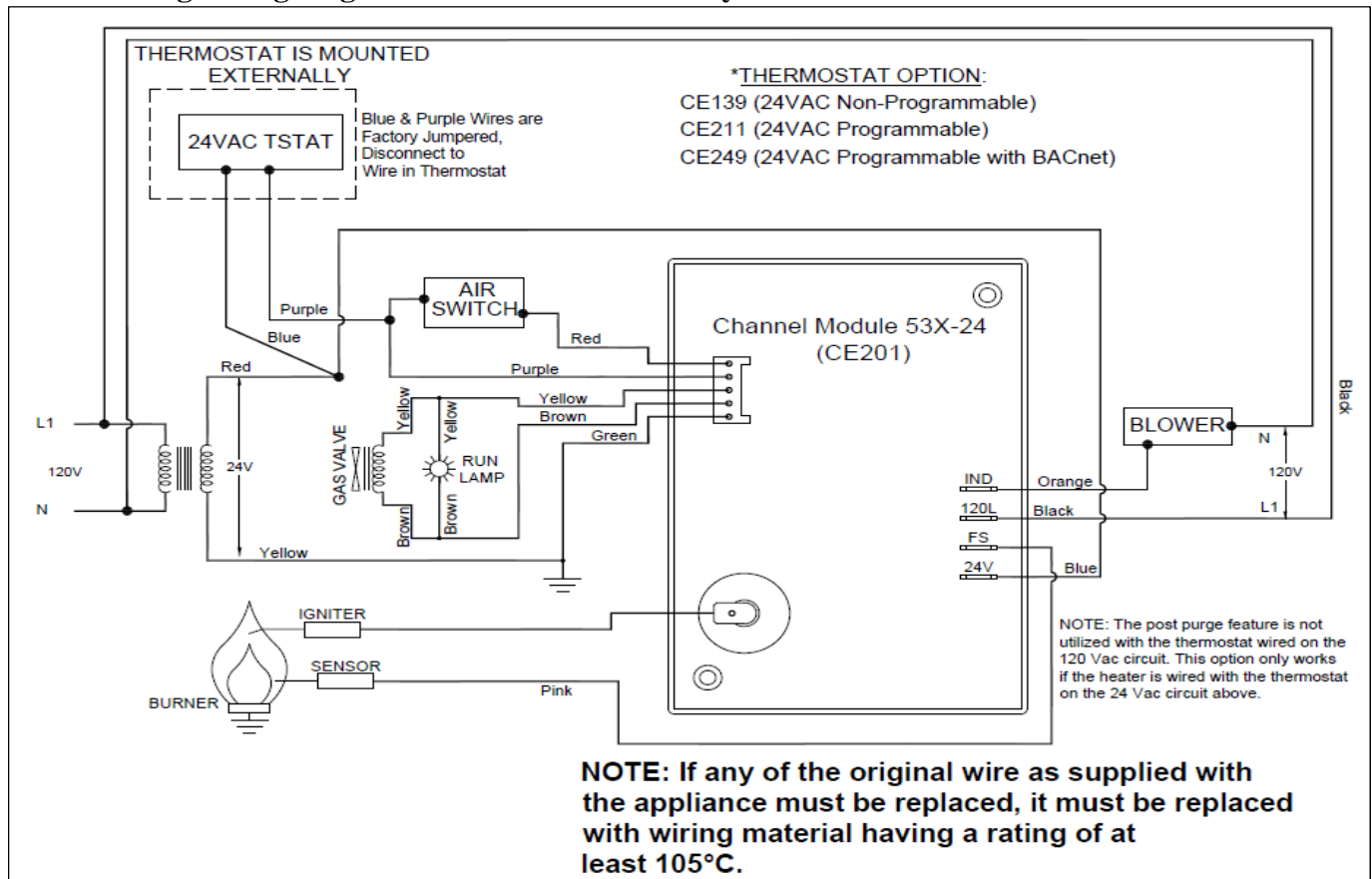
Figure 31: UXR Wiring Diagram
