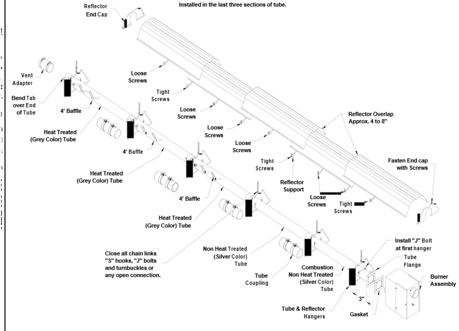
Figure 5: Installation Configuration for 100,000 BTU Model
