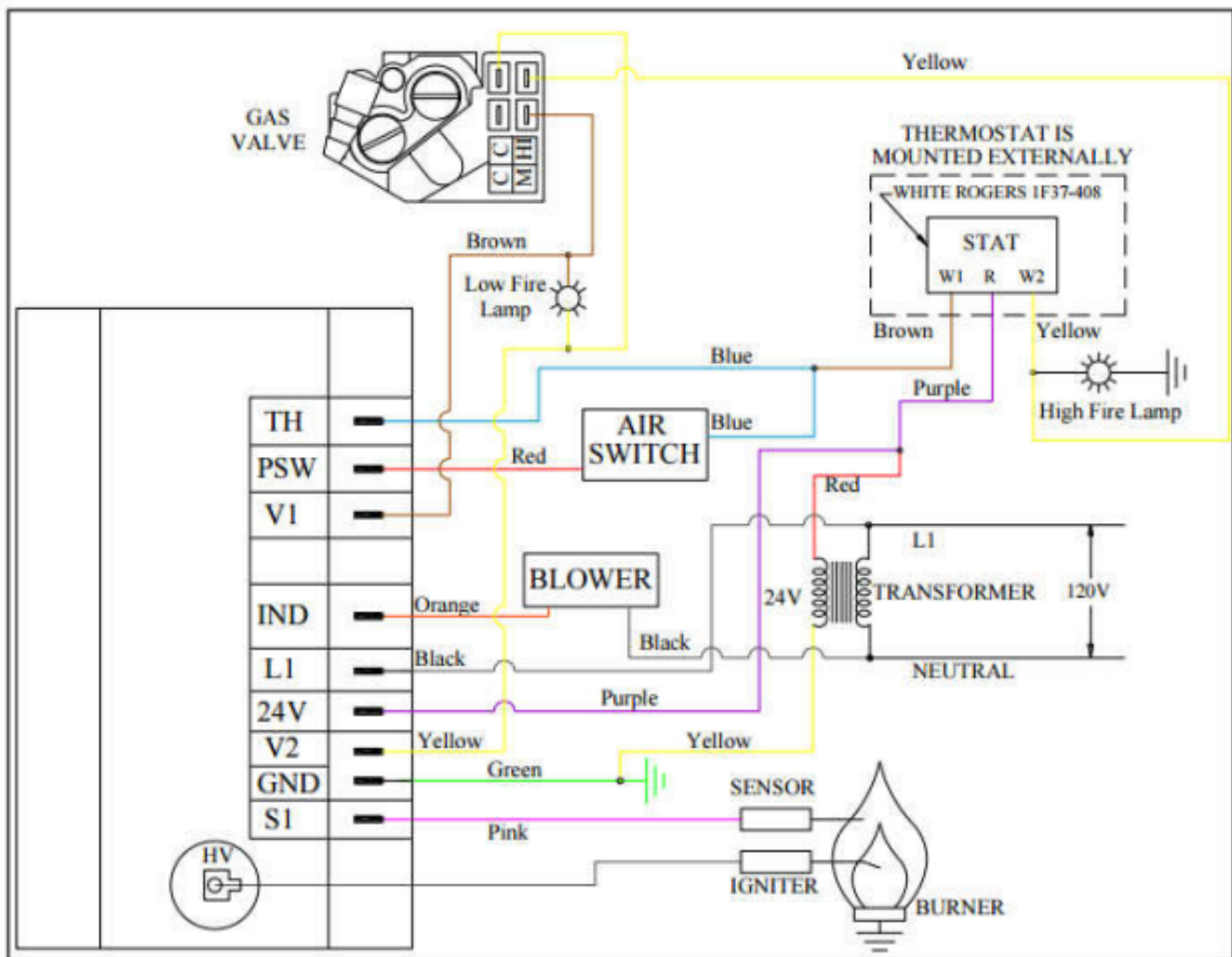
Wiring Diagram Series 750 LTX
